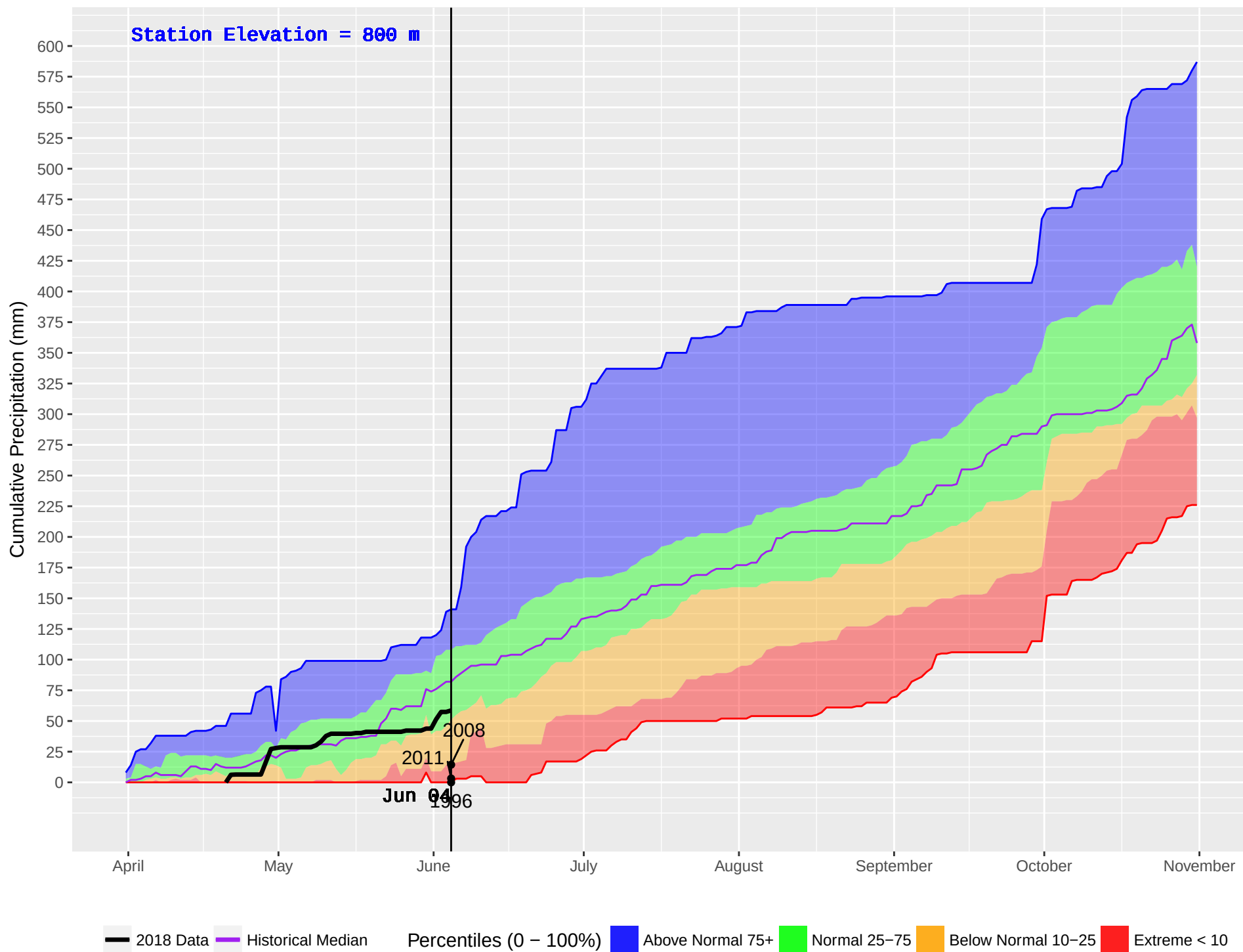
GOLD HILL (379) : Historical (1979–2016) and Current (2018) Noon Cumulative Precipitation
