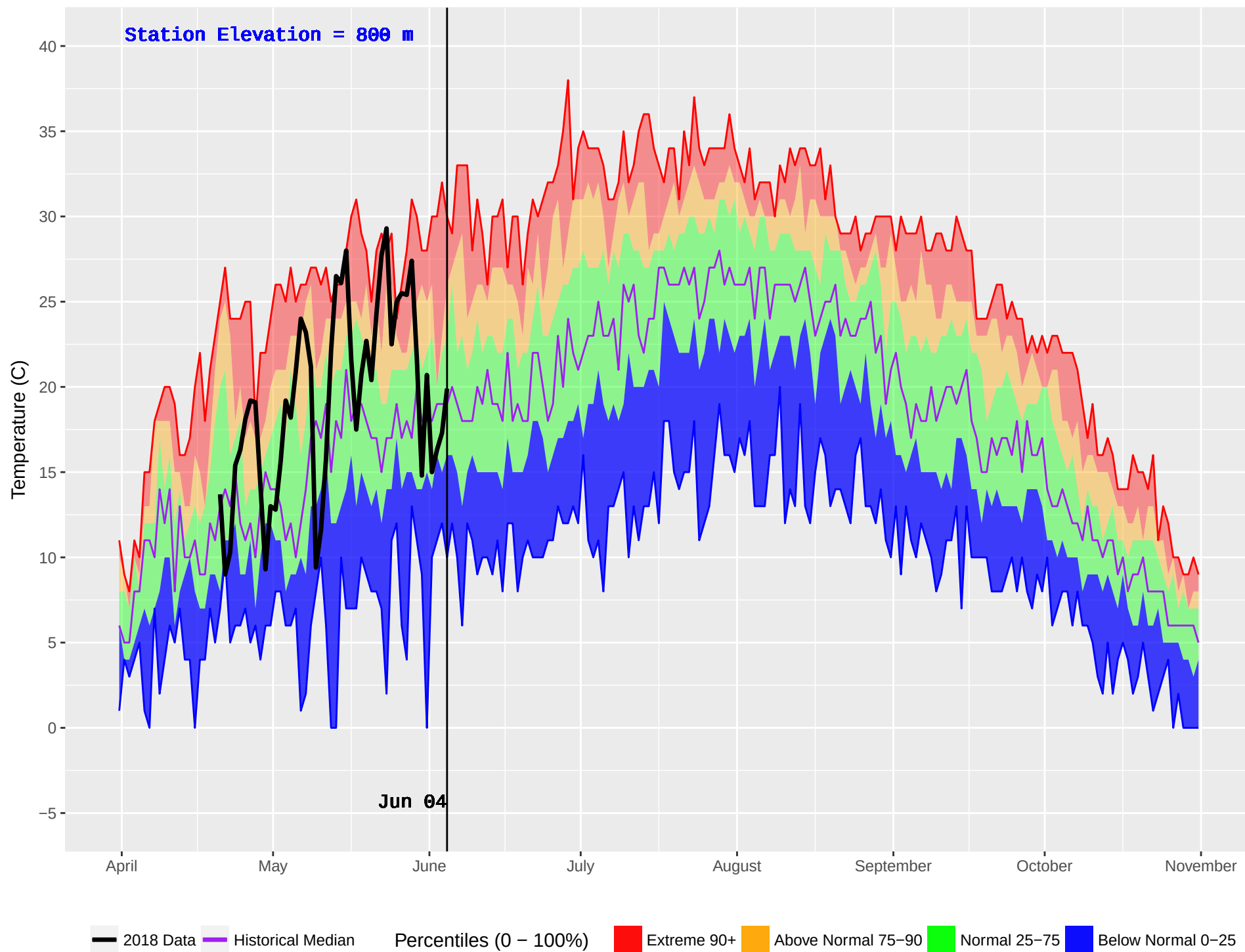
GOLD HILL (379) : Historical (1979–2016) and Current (2018) Noon Temperature
