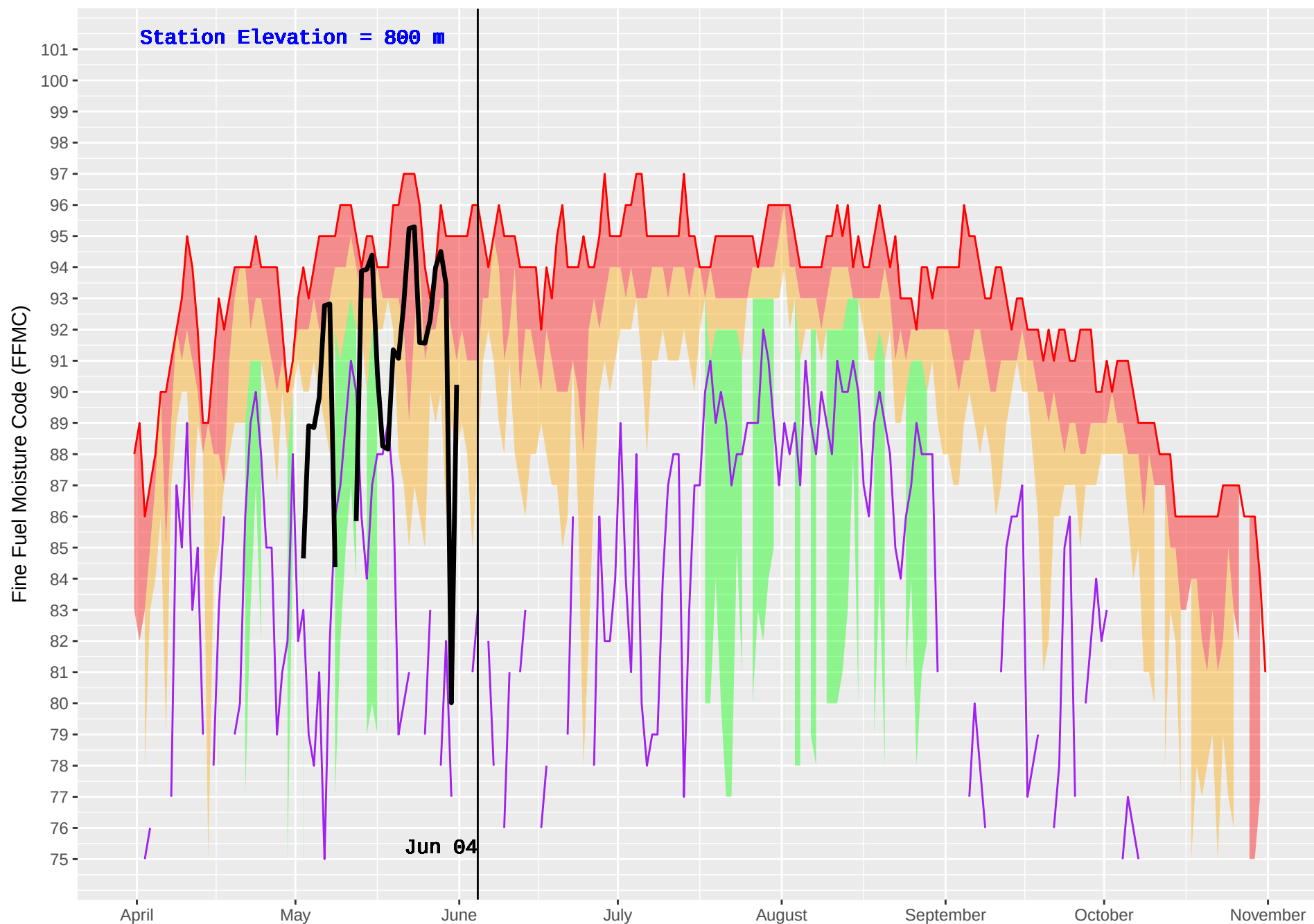
GOLD HILL (379) : Historical (1979–2016) and Current (2018) Noon Fine Fuel Moisture Code (FFMC)
