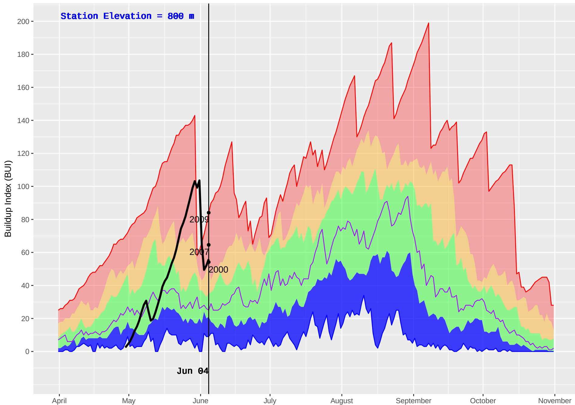
GOLD HILL (379) : Historical (1979–2016) and Current (2018) Noon Buildup Index (BUI)
