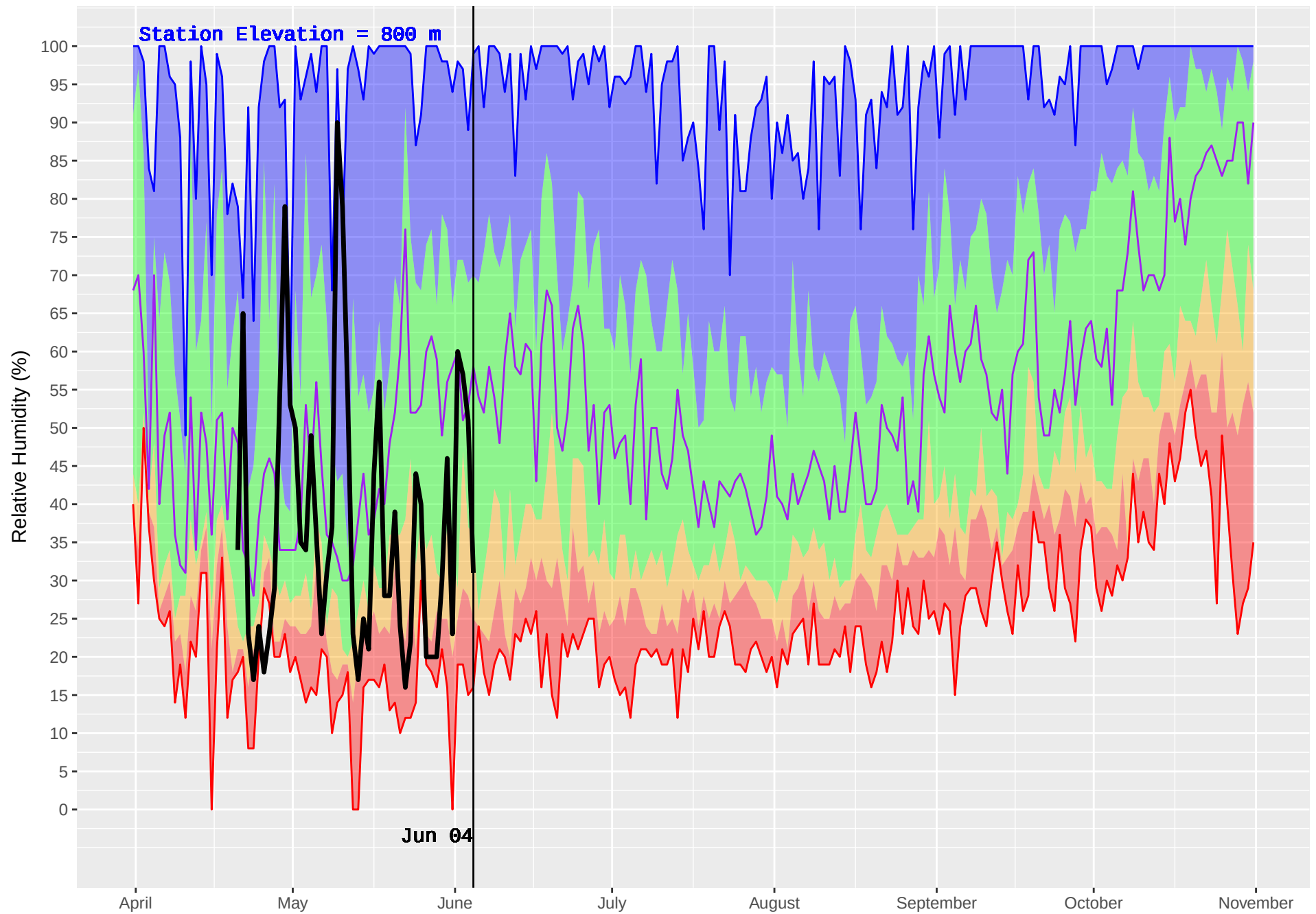
GOLD HILL (379) : Historical (1979–2016) and Current (2018) Noon Relative Humidity
